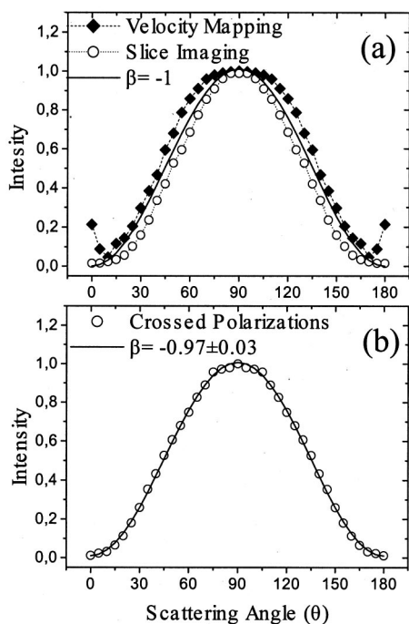
FIG. 7. (a) Angular distributions obtained with conventional and with slice imaging when the polarizations of the photolysis and probe lasers are parallel. Also shown is a fit to both data for \beta = -1 . (b) Angular distributions obtained with slice imaging when the polarizations of the photolysis and probe lasers are crossed.
