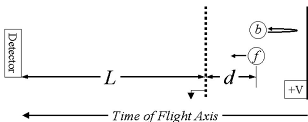
FIG. 1. Typical ion imaging setup, consisting of a homogeneous extraction field \bar{E} , a drift region of length L , and a position-sensitive detector (a phosphor screen combined with a CCD camera).
